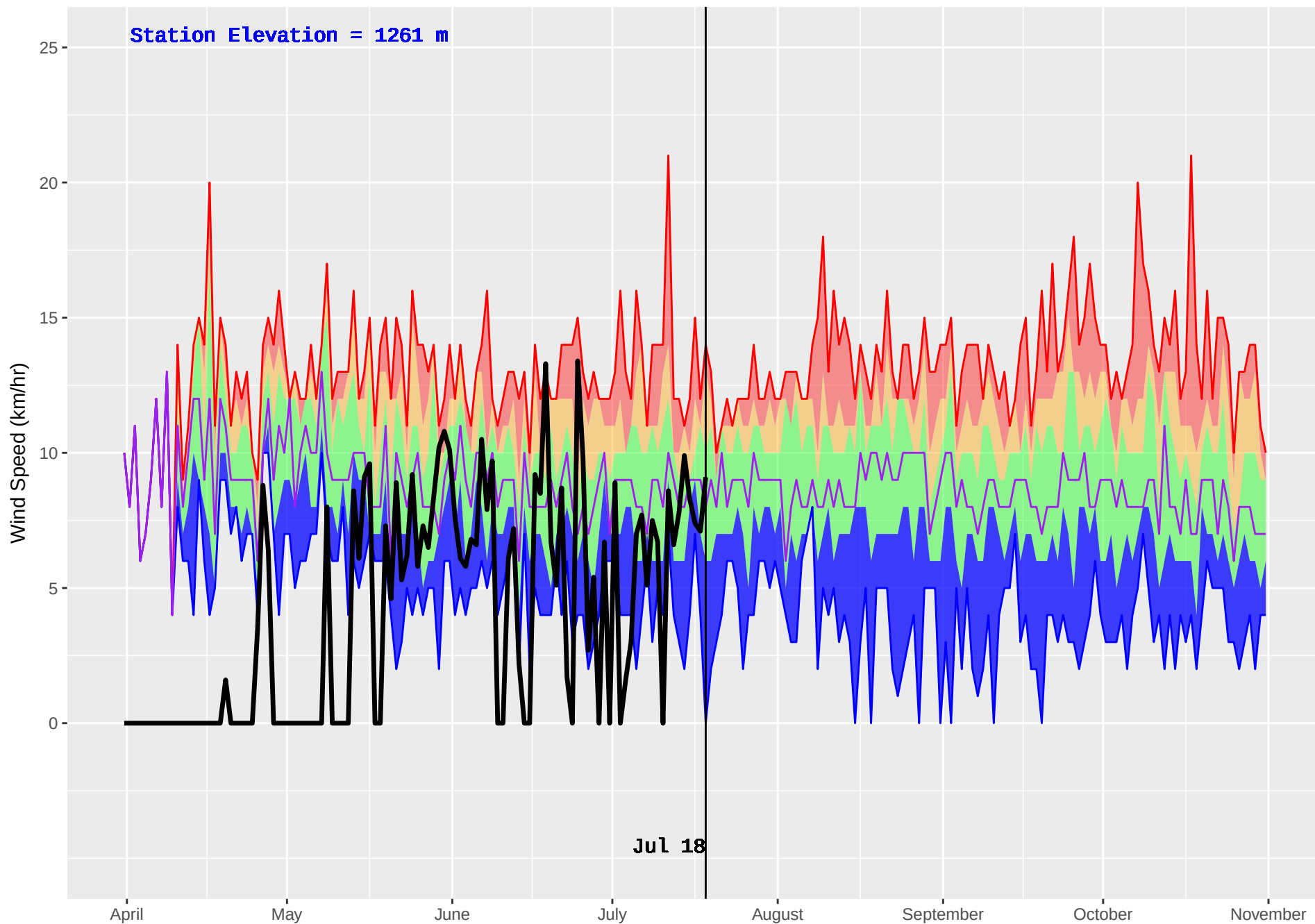
IDA BELL LAKE 3 (876) : Historical (2004–2016) and Current (2018) Daily Wind Speed
